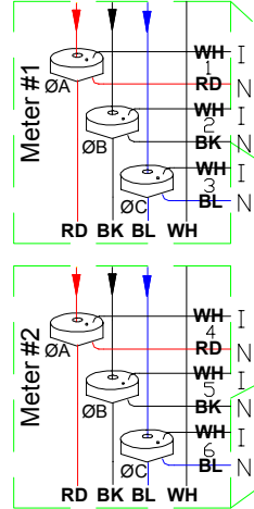
Diagram 1. Current Transformers installed inside tenant breaker panel.
