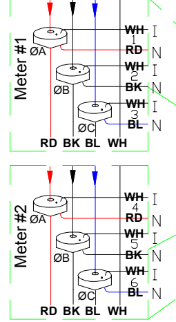
Diagram 1. Current Transformers installed inside tenant breaker panel.
