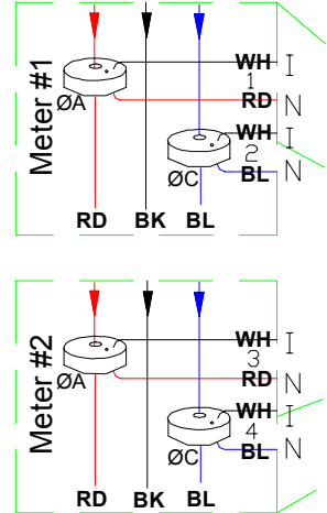
Diagram 1. Current Transformers installed inside tenant breaker panel.
